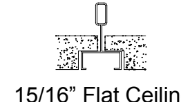
15/16" Flat Ceiling
