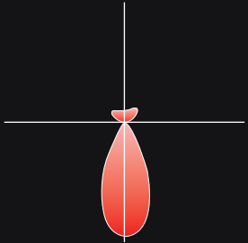
Micro Reflector (60°) UGR<15
