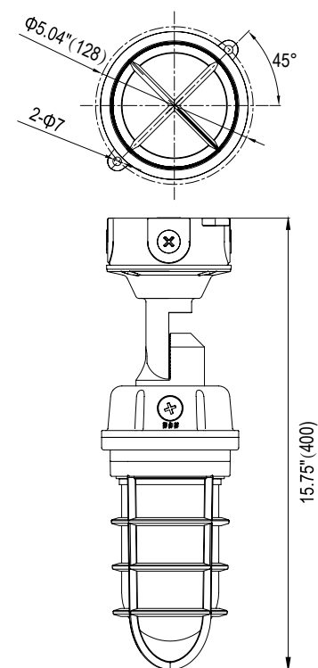
Ceiling Mount
