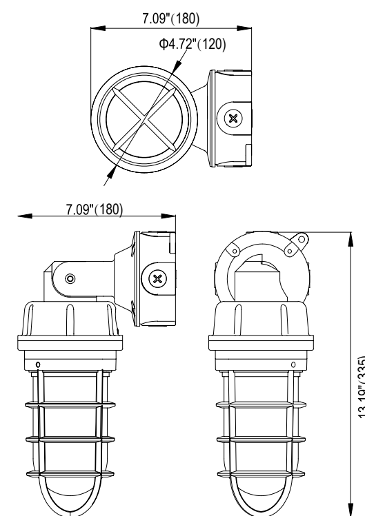
Wall Mount
