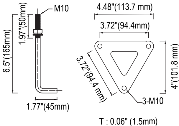
ANCHOR BOLTS AND PLATE
