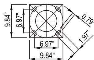
Pole Base
