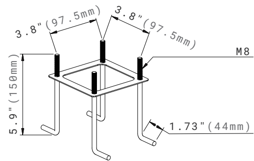
ANCHOR BOLTS
