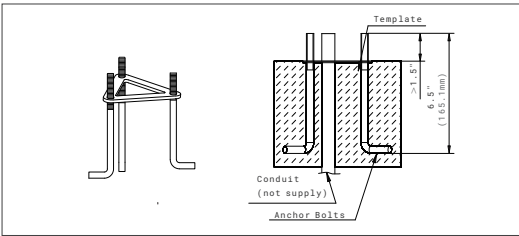
ABMK-SRBD-R Anchor Bolts Mounting Kits.
