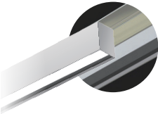
Regressed Lens
