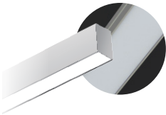
Regressed Lens
