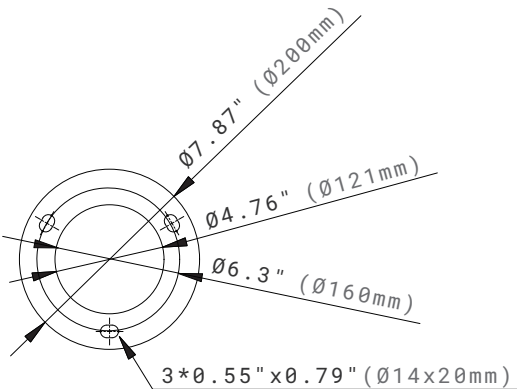
Base Plate
