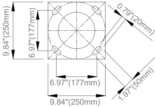
BASE PLATE
