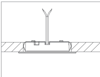
Recessed Mount
