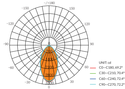
AVERAGE BEAM ANGLE(50%): 57.4 DEG
