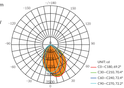
AVERAGE BEAM ANGLE(50%): 71.0 DEG
