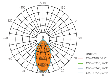
AVERAGE BEAM ANGLE(50%): 56.9 DEG
