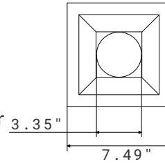
White Ring Metal Reflector
