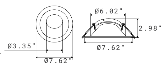
White Ring Metal Reflector
