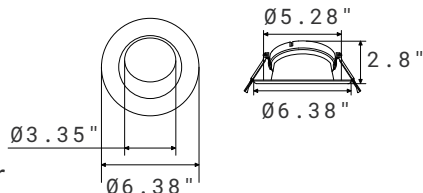
White Ring Metal Reflector
