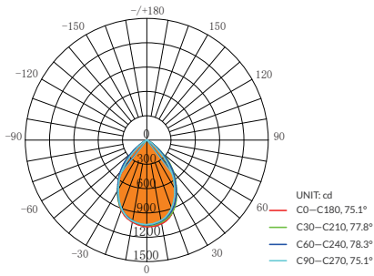
AVERAGE BEAM ANGLE(50%): 76.6 DEG
