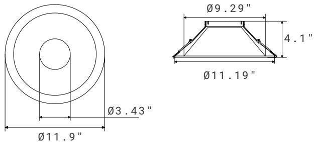
White Ring Metal Reflector
