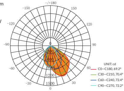
AVERAGE BEAM ANGLE(50%): 71.0 DEG
