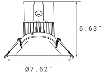
6" Round Wall Wash Trim
