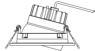
Tilt Angle. 30° Fixture
