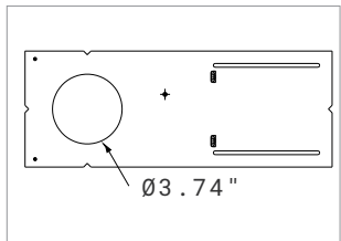
POR04-RIP-N Rough-in plate.
