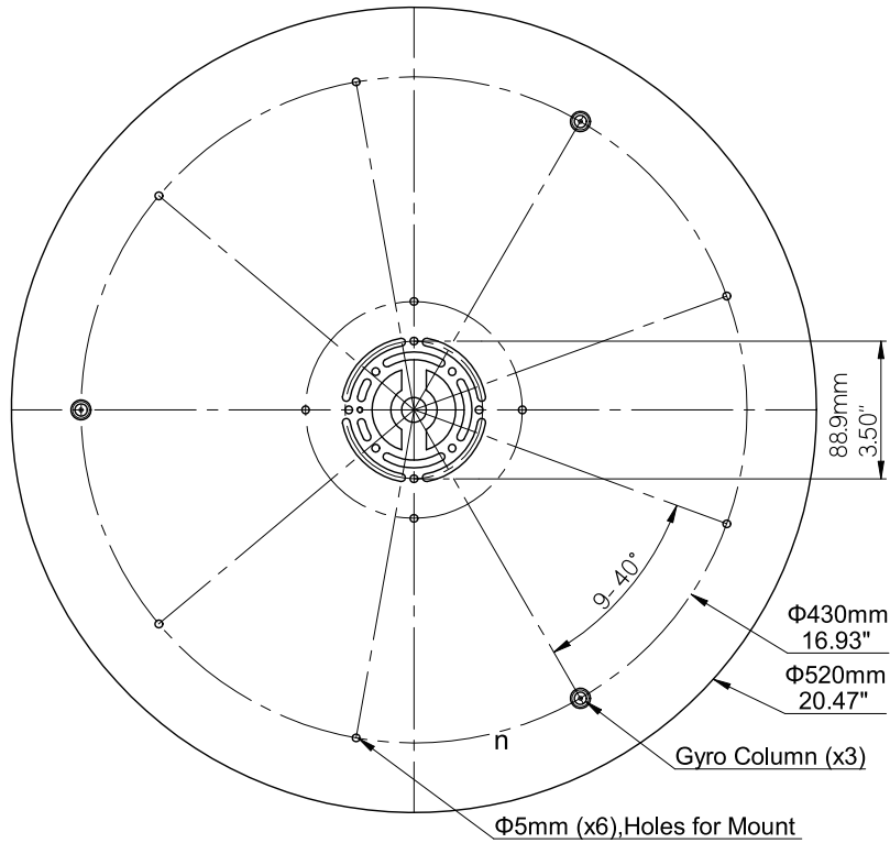
Surface mount plate for 24" Focus Light
