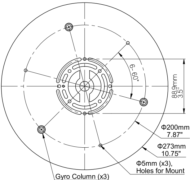
Surface mount plate for 24" Focus Light
