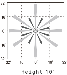
PIR Coverage Top View
