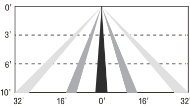
PIR + Ultrasonic Coverage Top View
