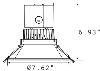
6" Round Trim
