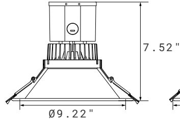
8" Round Trim
