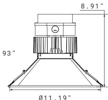
10" Round Trim
