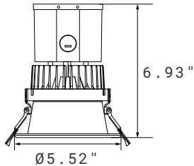
4" Round Trim
