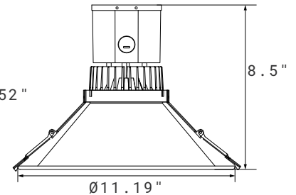
10" Round Trim
