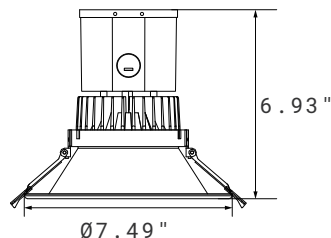
6" Square Trim
