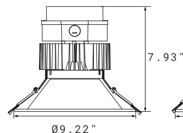
8" Round Trim
