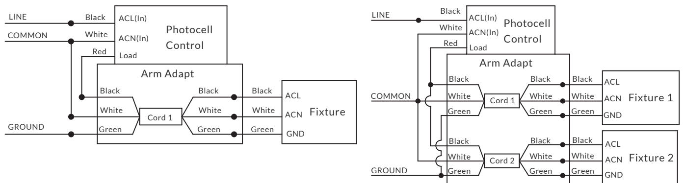
Wiring Diagram For 120-277V/347V/480V Photocell Control
