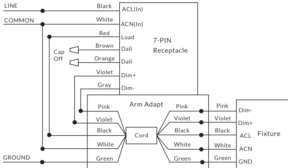
Wiring Diagram For 120-277V/347V/480V 7-PIN Receptacle
